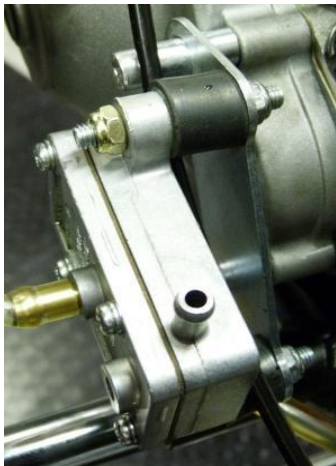
Foto of the frame with the section of the support for the fuel pump (fuel pump mounted)
